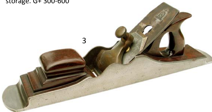
3 Spiers 20 1/2" dovetailed steel jointer plane with protruding toe and heel. Close to fine with beautiful rosewood in-fill and handle. One small scratch on front bun, minor rust/pitting marks on sole. G+ $ 600-1,200
