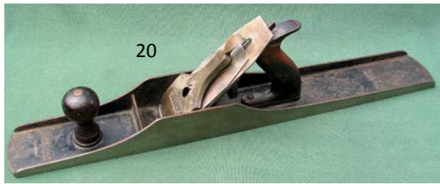
20 Stanley 608 Bedrock jointer, SW vintage. Handle spur glued, approximately 60% japanning intact, good SW cutter. G $ 150-300
