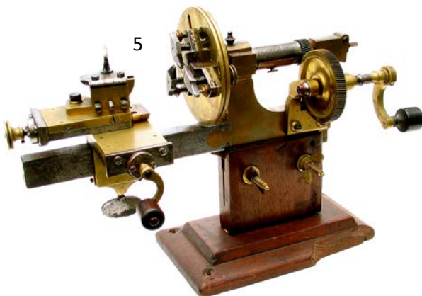
5 Rare Swiss watchmaker's mandrel lathe, brass and steel on mahogany base. Base loose in centre and chipped on one side. Minor rust spots on some of the steel parts. 18" x 11" x 8" G $ 350-700
