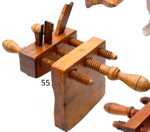
55 European style triple-stemmed circular Cooper's grooving router with fence and nice border decorations. Marked BALOGH Szerszam VAC. Some bruising to wedges and minor age related nicks. G+ $ 100-200
