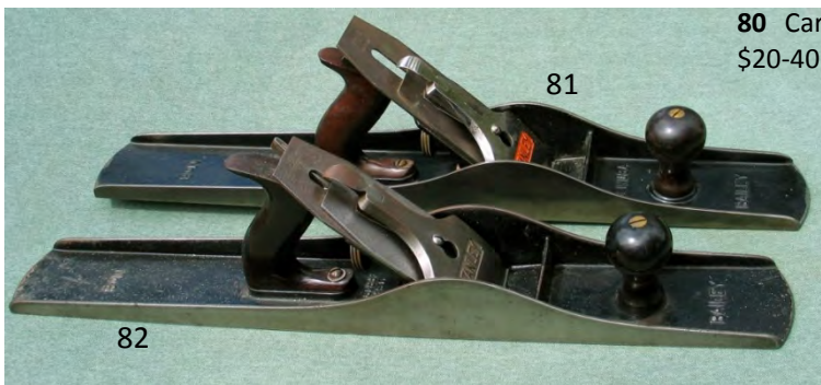
81 Stanley 8C with SW cutter, keyhole lever cap and very good wood. Over 95% japanning intact. F $ 150-250
