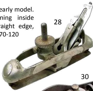
28 Stanley 20 circular plane. Nickel plating 95%. Full Pat 92 cutter. Very good, early plane. G+ $ 120-200
