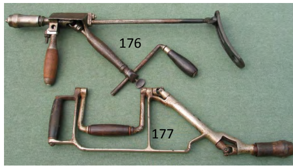
176 Impressive 20" breast drill with Miller Falls chuck, adjustable plate and front handle. I suspect some restoration work but hardly noticeable. G $ 70-140
