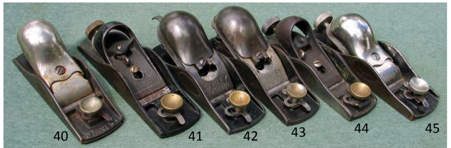
40 Stanley 18 knuckle-joint block plane. All parts correct for SW vintage. Minor rust on sole. G+ $ 20-40
