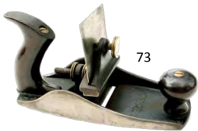
73 Stanley 112 scraper plane. VG wood, most japanning intact. Unmarked cutter. G+ $ 100-200
