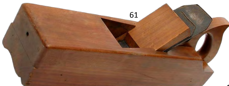
61 Large and heavy cormier wood crown moulder with unusual double irons that are wedge only (not screwed together like back iron and cutters). 16" x 3 1/2" and cuts a 3" ogee. Maker's mark on side: Aux Mines de Suede, Paris. G+ $ 70-150
