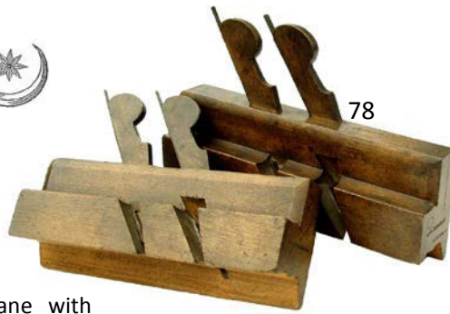
78 Rare pair of Mathieson double iron sash moulders marked 1 & 2 on toe. Early Edinburgh mark. G+ $ 100-200
