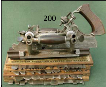
200 Stanley 55 combination plane. Basic unit without auxi tower but a good set of 51 out of 52 cutters. Perfect user tool. G $ 150-250
