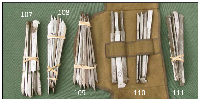
107 Set of No 1-8 Mathieson plough plane cutters. All G+ $ 30-60
