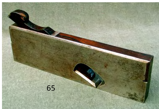
65 dovetailed 3/4" Spiers steel rebate plane with rosewood infill and rosewood wedge. Cutter is very good but not original. Owner's marks front and back. G $ 70-140
