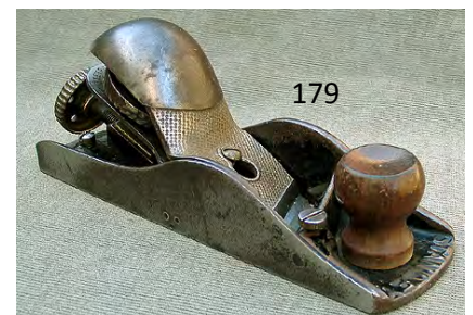
179 Stanley 140 rabbet & block plane, complete with fence. One fence screw is not original. Minor rust spots, most japanning intact, good cutter. G $ 70-150
