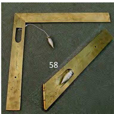
58 French hinged 6" folding brass square with integrated plumb bob marked ligne aplomb plus other markings. G $ 25-50
