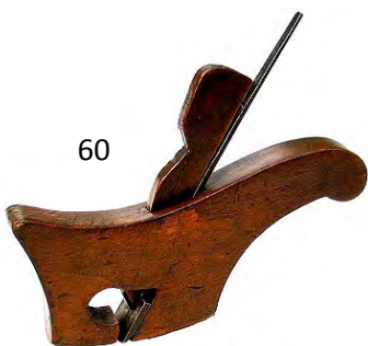
60 Tailed Dutch coachmaker's plane with round and compassed sole. 6 1/4" long. G+ $ 40-80
