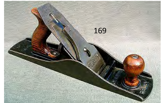
169 Stanley 5 1/2 jack plane made in USA. Over 95% japanning intact, full cutter, good beech handle and knob. Clean plane. G+ 50-100
