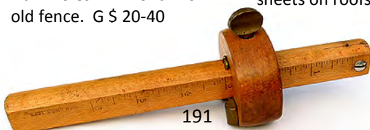
191 Stanley 164 beech marking gauge with brass insert on fence and brass plate for convex work. Pat 73 on slide and on brass plate. G $ 25-50
